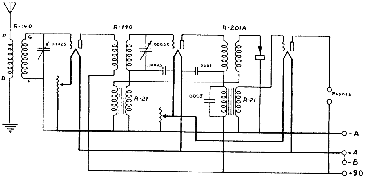
ALL-AMAX SENIOR
